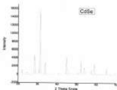
Fig. 2. X-ray diffraction spectra of CdSe nanoparticles Synthesized, by ultrasonic irradiation for 40 min.
